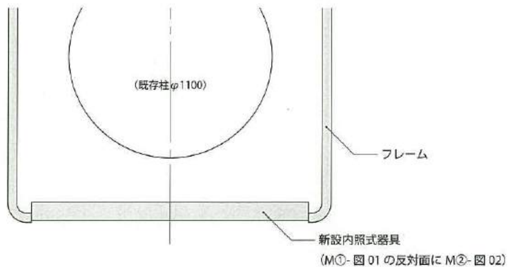
M①-図01 器具外形寸法H2200×W1750
