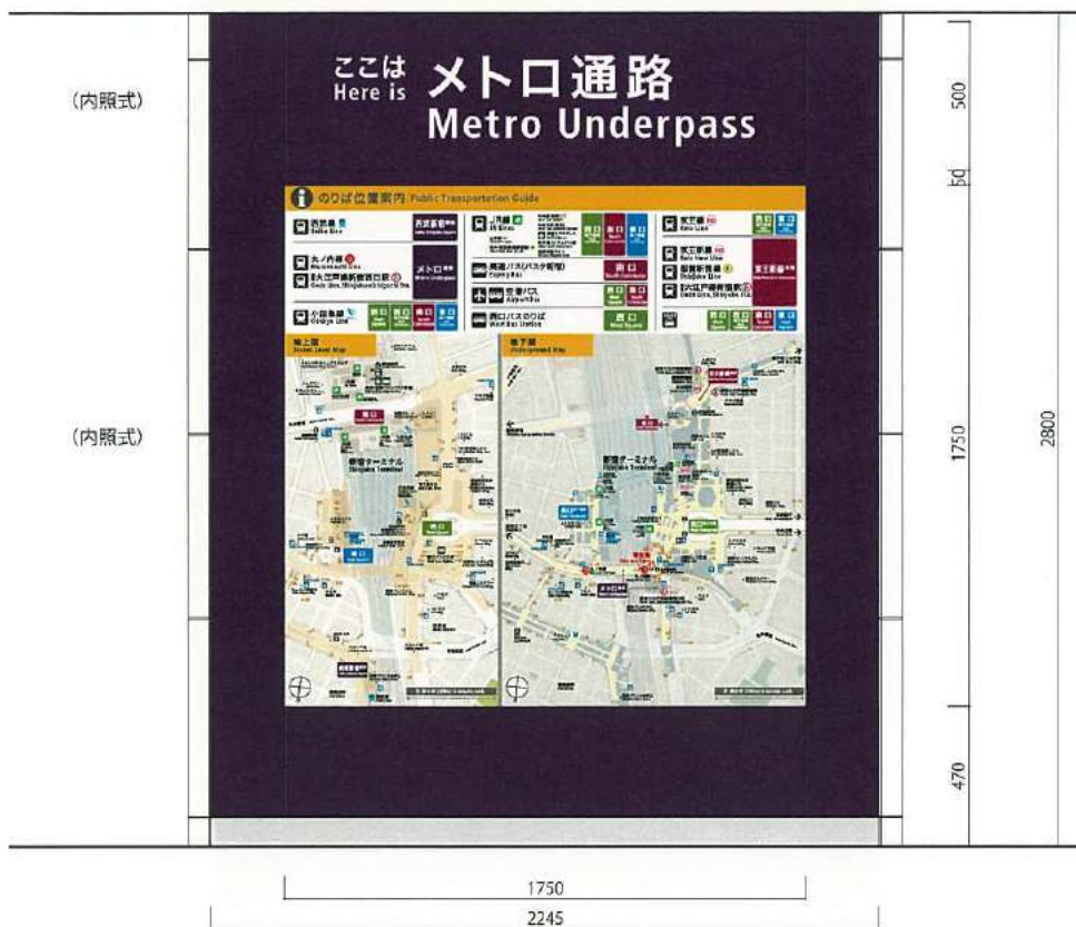
M①-図03 器具外形寸法H2800×W2245
