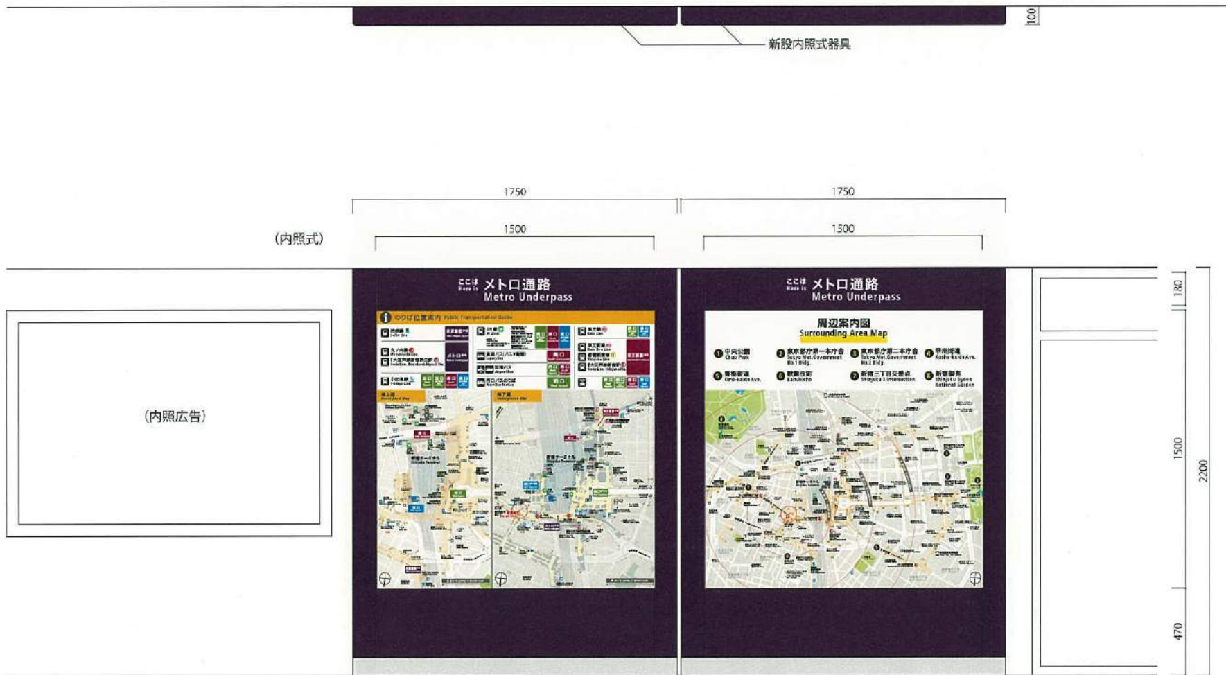
M②-図03 器具外形寸法H2200×W1750
