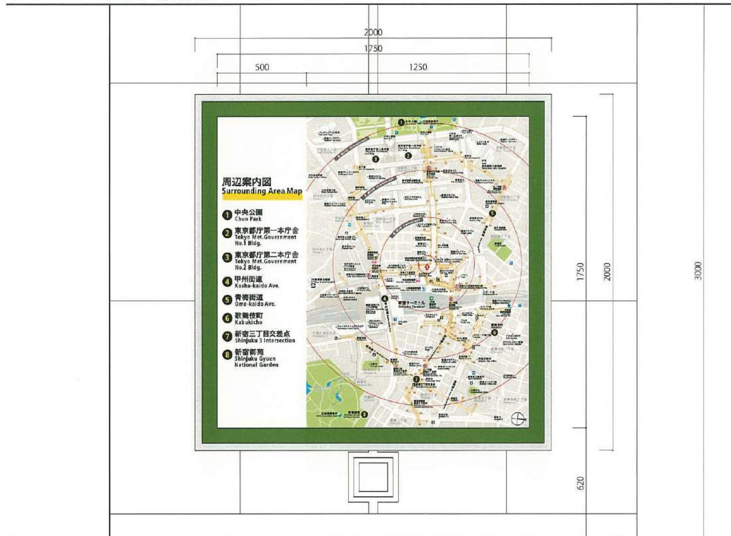
C-図07 器具外形寸法H2000×W2000
